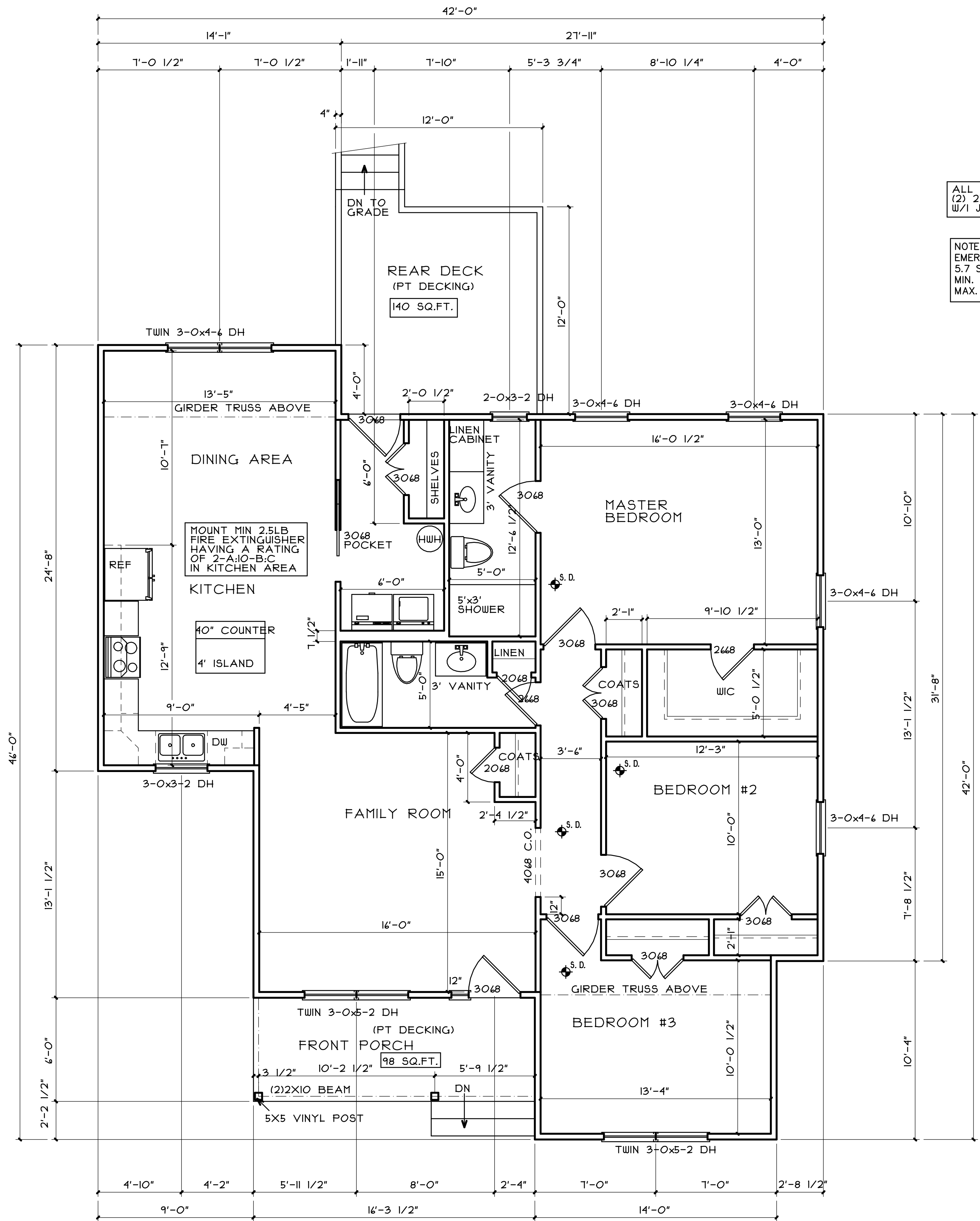
FIRST FLOOR PLAN 1,461 SQ.FT.
