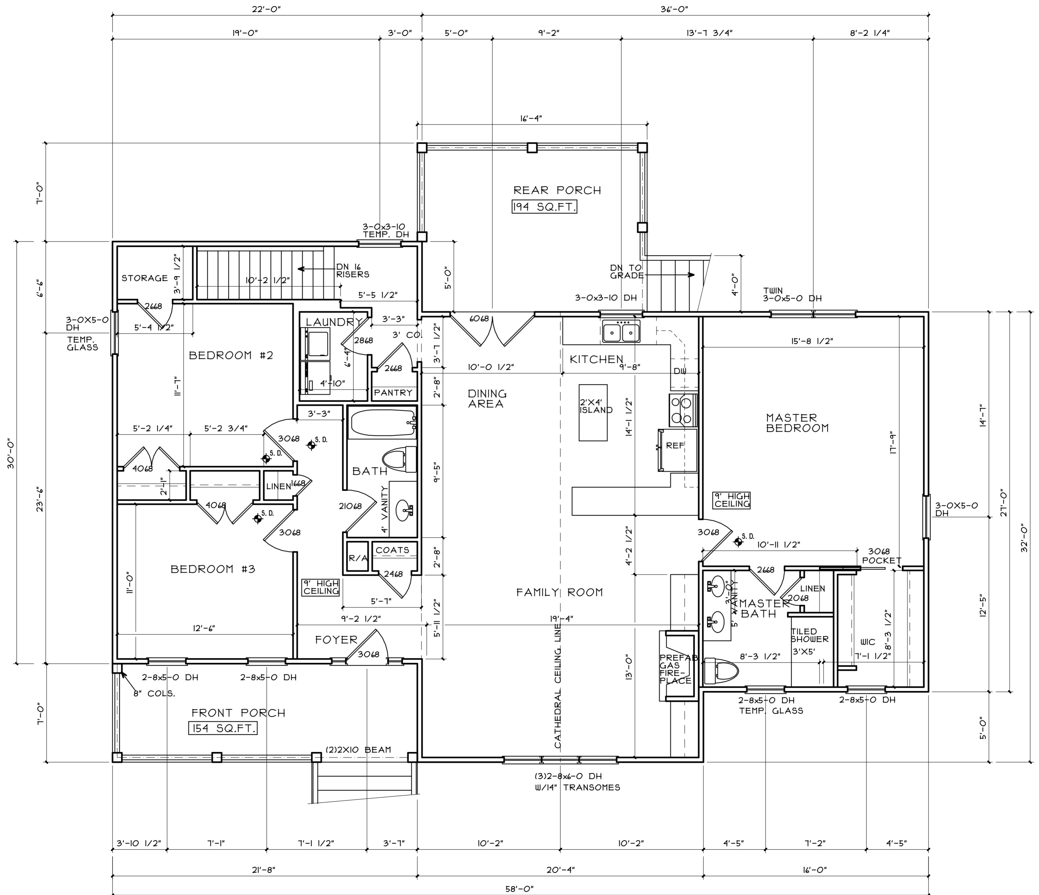
FIRST FLOOR PLAN 1,134 SQ.FT.
